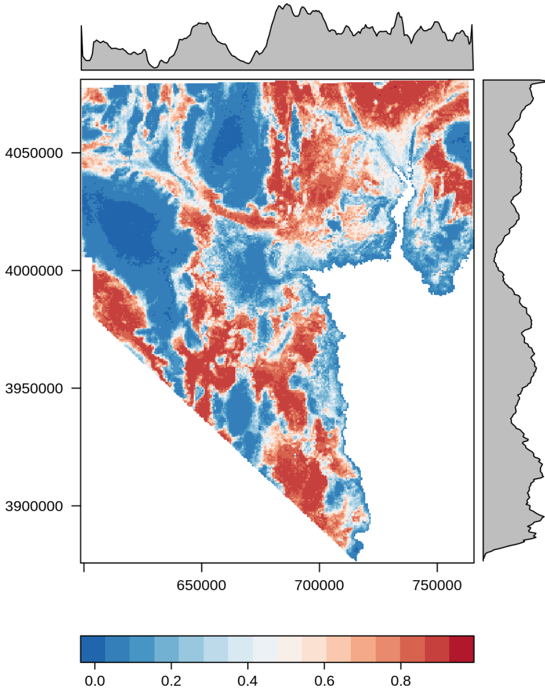
Figure A.14-7. SDM map for Mojave Desert tortoise Ensemble model for Clark County, NV.
