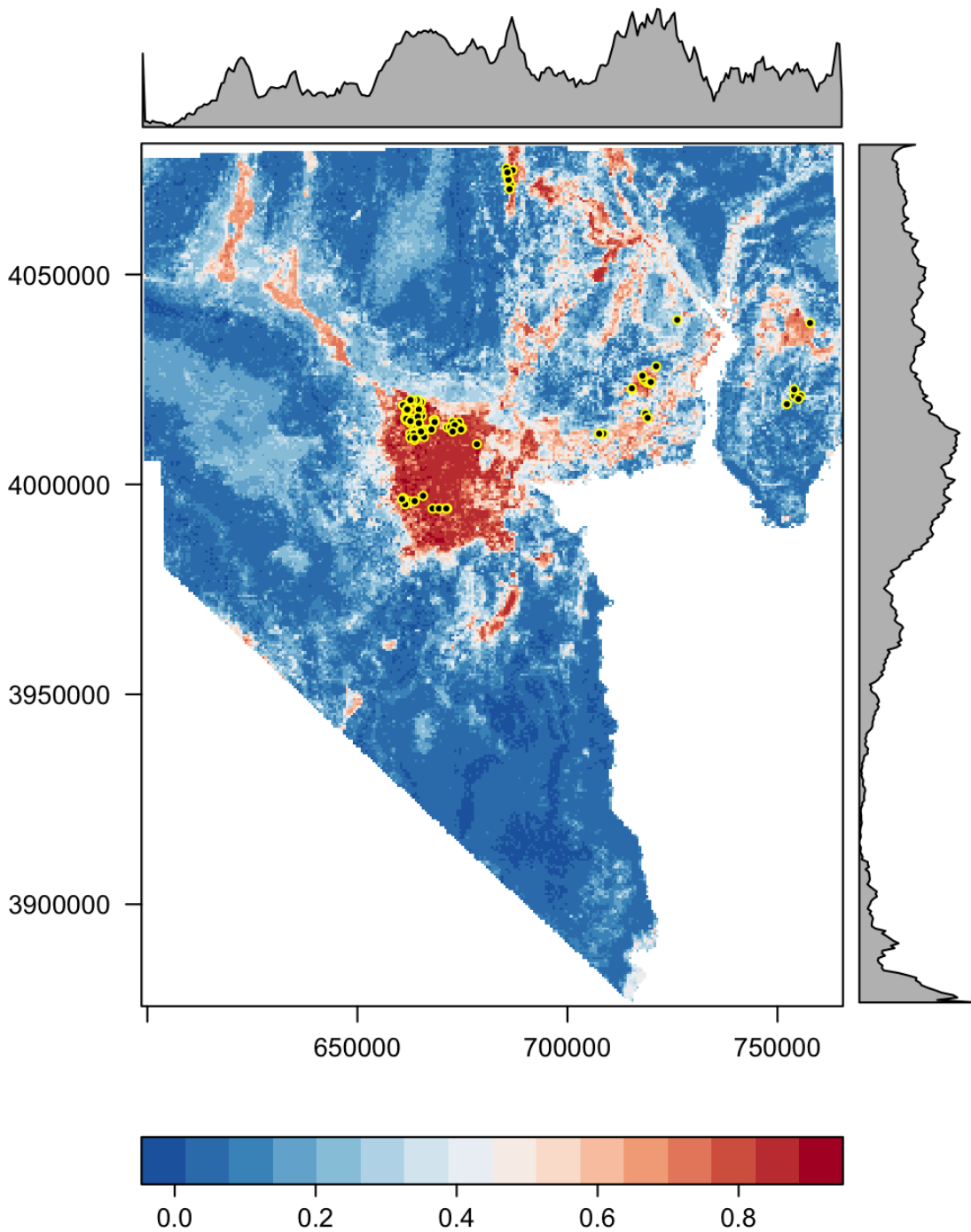
Figure A.8-7. SDM map for Las Vegas buckwheat Ensemble model for Clark County, NV.
