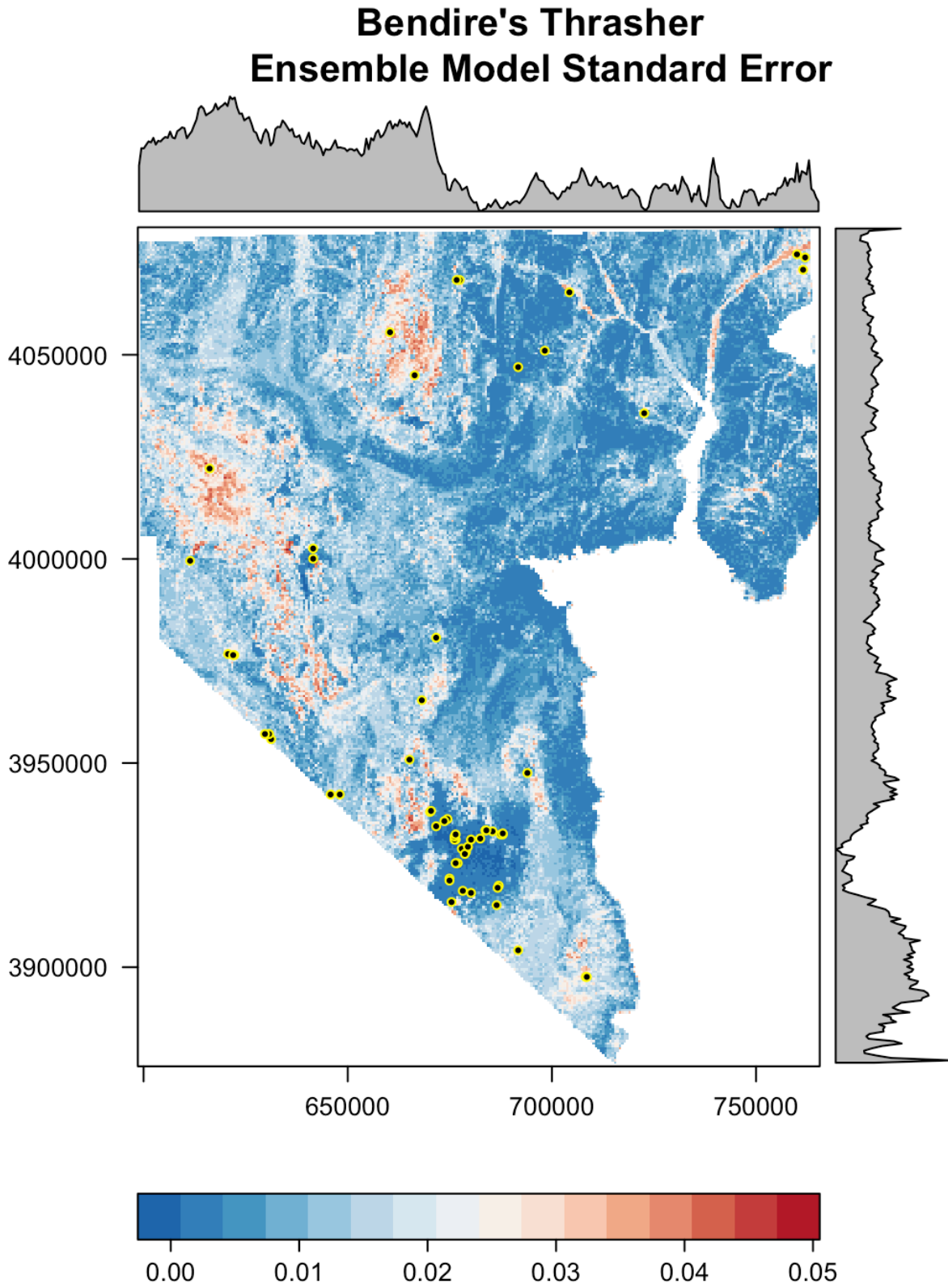
Figure A.23-8. Standard Error map for the Bendire's thrasher ensemble model for Clark County, NV.
