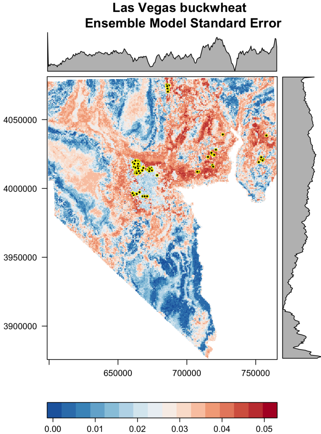
Figure A.8-8. Standard Error map for the Las Vegas buckwheat Ensemble model for Clark County, NV.
