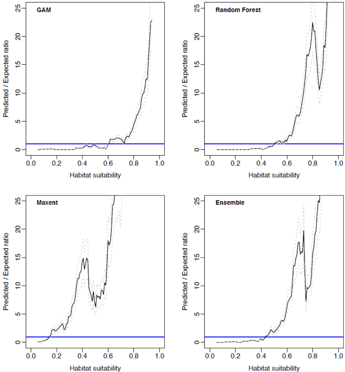
Figure A.6-3. Continuous Boyce Indices for silverleaf sunray models for each of three modeling algorithms used (GAM - upper left, RF - upper right, MaxEnt - lower left), and an Ensemble model averaging the three (Lower Right).
