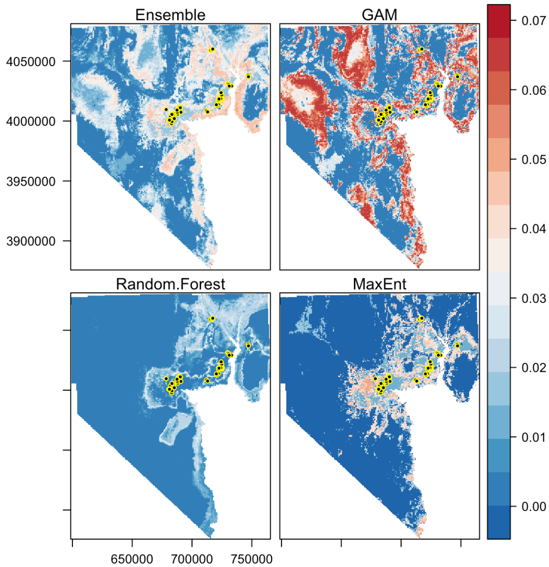
Figure A.1-2. Standard error maps for sticky ringstem models for each of three modeling algorithms used (GAM - upper right, Random Forest – lower left, MaxEnt - lower right), and an Ensemble model averaging the three (upper left).
